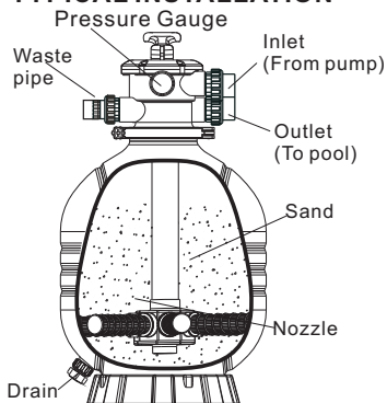
TYPICAL INSTALLATION
